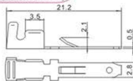
HX28050-RT(DJ611-2.8x0.5A-B)
